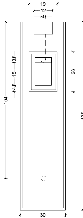
VISTA FRONTAL
